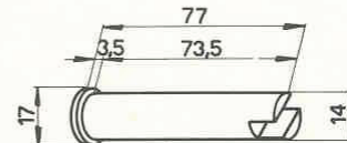
Chasse-pointe 120-C-9
