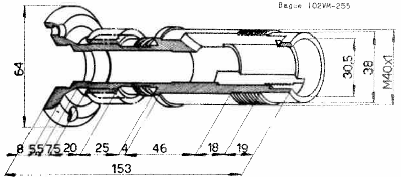
Manchon 102VM-253
