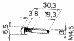
Vis 102-611-Q
