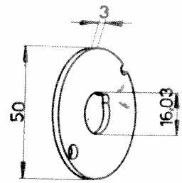
Bague 102VM-6116
