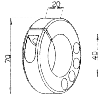
Bague 120-TS-44
