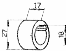
Bague 102VM-1716
