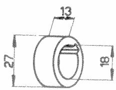
Bague 102VM-1723
