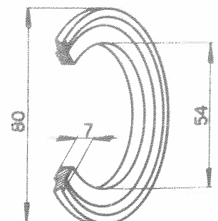
Bague 120 PER-14
