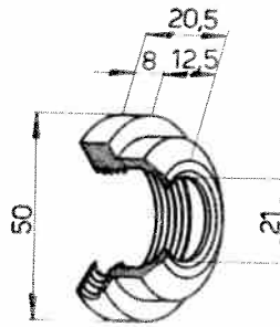
Ecrou 102-CH-189
