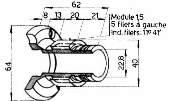
Vis-sans-fin 102VM-103
