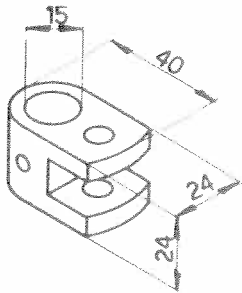
Fourche 102VM-804
