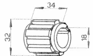
Manchon 102VM-6151
