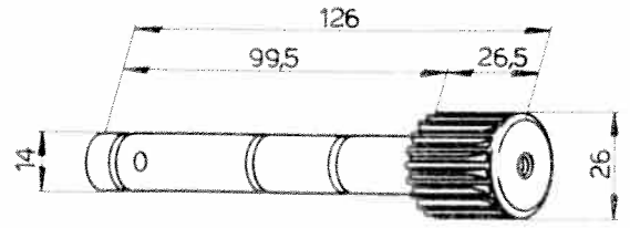
Pignon 102VM-6069
