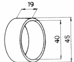
Bague 102-PER20-11
