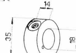
Bague 102VM-754
