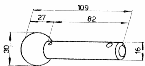
Rotule 102VM-684
