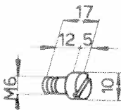
Vis de fixation 102VM-8085
