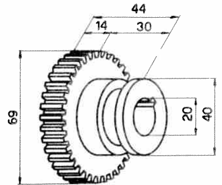
Engrenage 102-PER20-23
