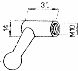
Poulet 102VM-745 Poignée 102VM-837
