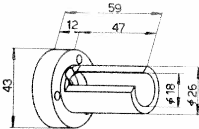
Douille 102VM-839
