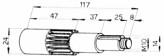
Pignon 102VM-757
