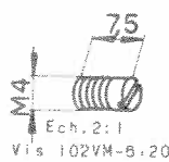
Vis 102VM-6.20
