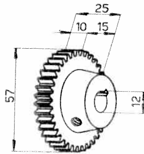
Engrenage 102VM-759
