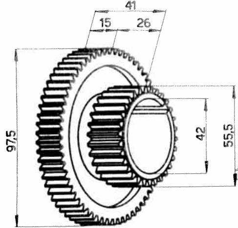
Engrenage 102-PER20-20
