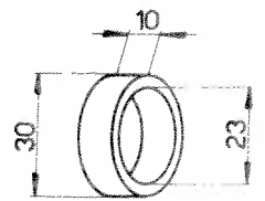
Bague 102VM-255
