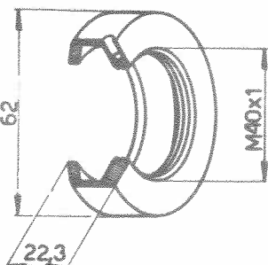
Bague 102VM-257
