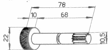
Pignon 102VM-163
