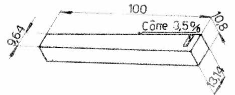
Lardon 102VM-829
