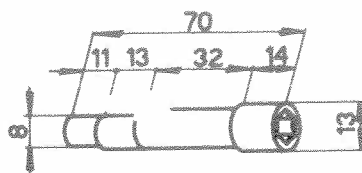
Eccentrique 102VM-356
