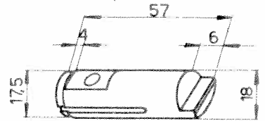
Verrou 102VM-840
