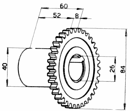
Engrenage 102VM-6031
