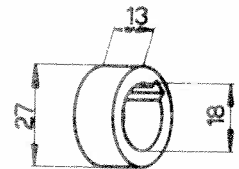
Bague 102VM-1723
