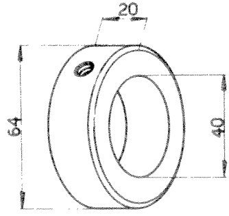
Bague 120-TS-32
