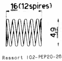
Ressort 102-PEP20-26
