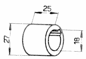
Bague 102VM-1717
