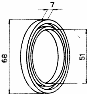
Bague 102-PER20-7
