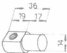
Ecrou 102VM-359
