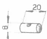
Piston 102VM-6117
