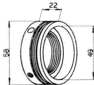
Ecrou-chicane 102VM-6175
