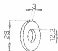
Bague 102VM-6115
