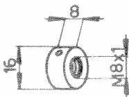
Ecrou 102VM-358
