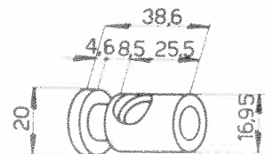
Tirant 102VM-354
