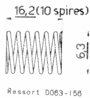
Ressort D083-158
