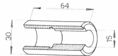
Outil 102VM-799
