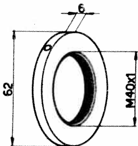
Bague 102VM-258
