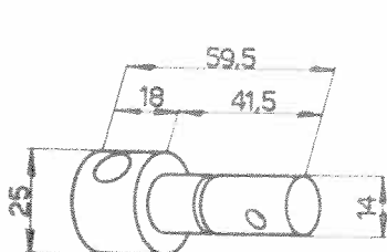
Pivot 102VM-6071
