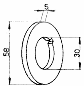
Bague 102VM-6037
