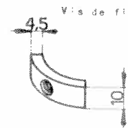
Segment 102VM-6084
