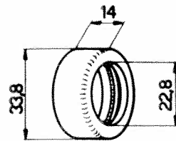
Bague 102-P20-9
