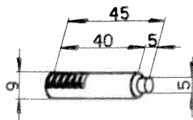
Piston 102VM-168
