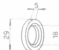
Bague 120VM-412
