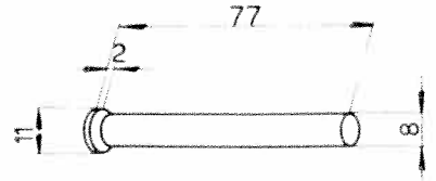
Chasse-pointe 102-608-G
