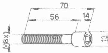
Vis 102VM-357
