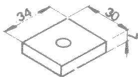
Plaque 102-VM-25
