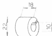
Bague 102VM-729
