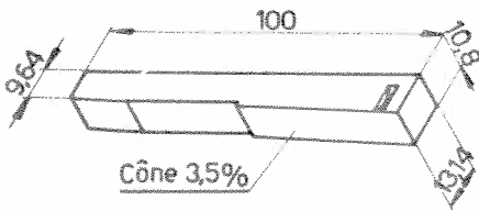
Lardon 102VM-830
