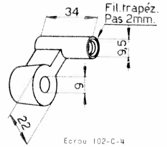
Ecrou 102-C-4
