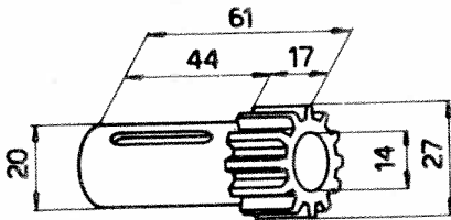
Pignon 102-PER20-21
