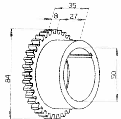
Engrenage 102VM-6058
