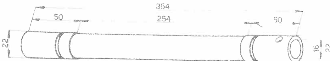
Broche 102VM-800
