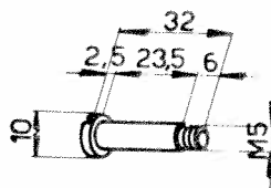
Pivot 102VM-841
