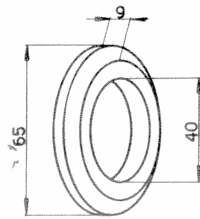
Bague 102VM-215
