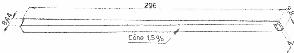
Lardon 102VM-742
