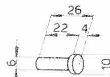
Piston 102VM-732
