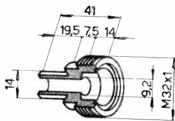
Manchon 102-CH-188
