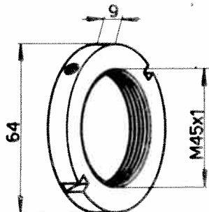
Ecrou 102-PER20-9a
