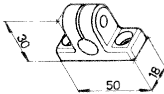
Support 120-VM-1383
