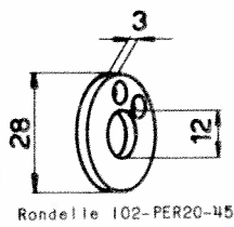
Rondelle 102-PER20-45
