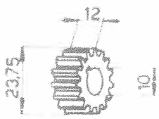
Engrenage 102VM-726
