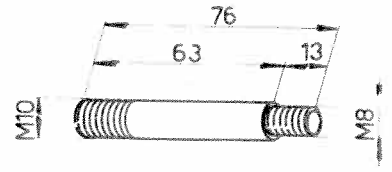
Goujon 102VM-834
