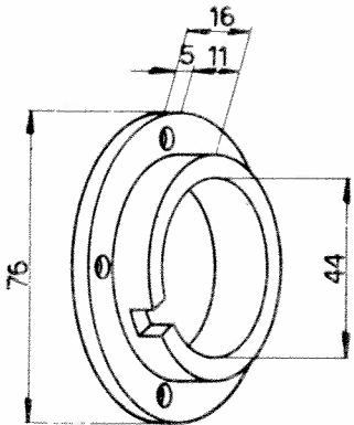
Bague 102VM-6180
