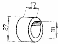
Bague 102VM-1716
