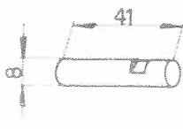
Piston 102VM-6117
