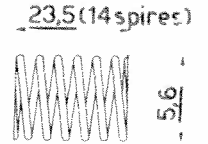
Ressort D058-38
