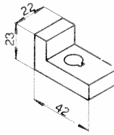
Bride 102VM-831
