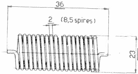
Ressort T230-3
