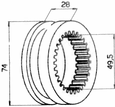
Engrenage 102-PER20-19
