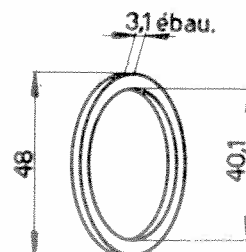
Bague 102-PER20-12
