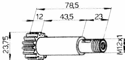
Pignon 102VM-728
