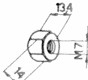
Ecrou 102-611-M
