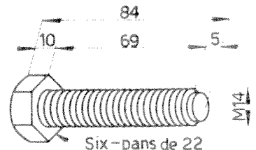
Bouton 120-TS-42
