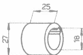
Bague 102VM-1717
