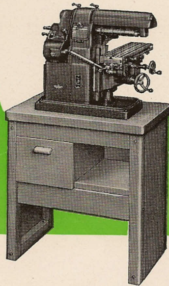
Atlas Series MF milling machine mounted on No. MI-750 hardwood floor cabinet.
